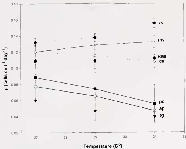
Figure 1. Growth rates of zooxanthellae isolated from 7 hosts at three temperatures. Points represent means; error bars represent \pm 1 SD ( n = 4 ). Data were obtained as increase in fluorescence over the 13-day growth period. Growth was logarithmic during this time. Fluorescence units were converted to cell density at the end of the growth period. Host: zs— Zoanthus sociatus , mv— Montipora verrucosa , cx— Cassiopea xamachana , KB8— Cassiopea KB8, pd— Pocillopora damicornis , ap— Aiptasia pulchella , tg— Tridacna gigas . The dotted lines represent algae in clade A, the solid lines algae in clade B, and the dashed line the alga in strain C.
